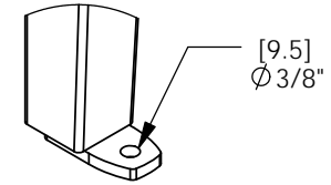
SURFACE MOUNT FOOT
